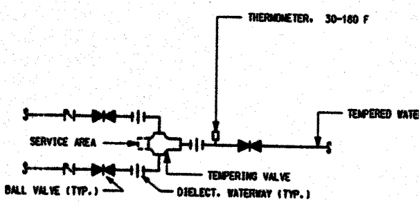
TEMPERED WATER VALVE DETAIL SCALE: NONE
