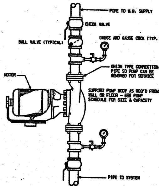
IN LINE CIRCULATING PUMP DETAIL SCALE NONE
