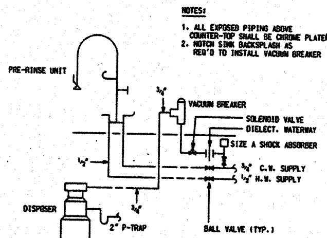
PRE-RINSE AND DISPOSER DETAIL SCALE: NONE
