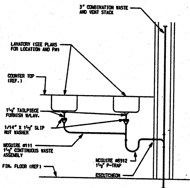
SIDE-BY-SIDE LAVATORY DRAIN DETAIL SCALE: NONE
