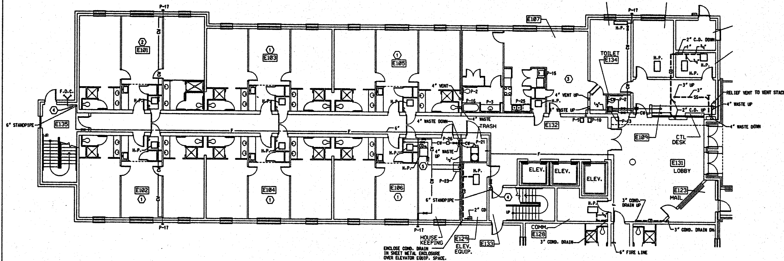
PLUMBING - FIRST FLOOR PLAN - PART 'A'
