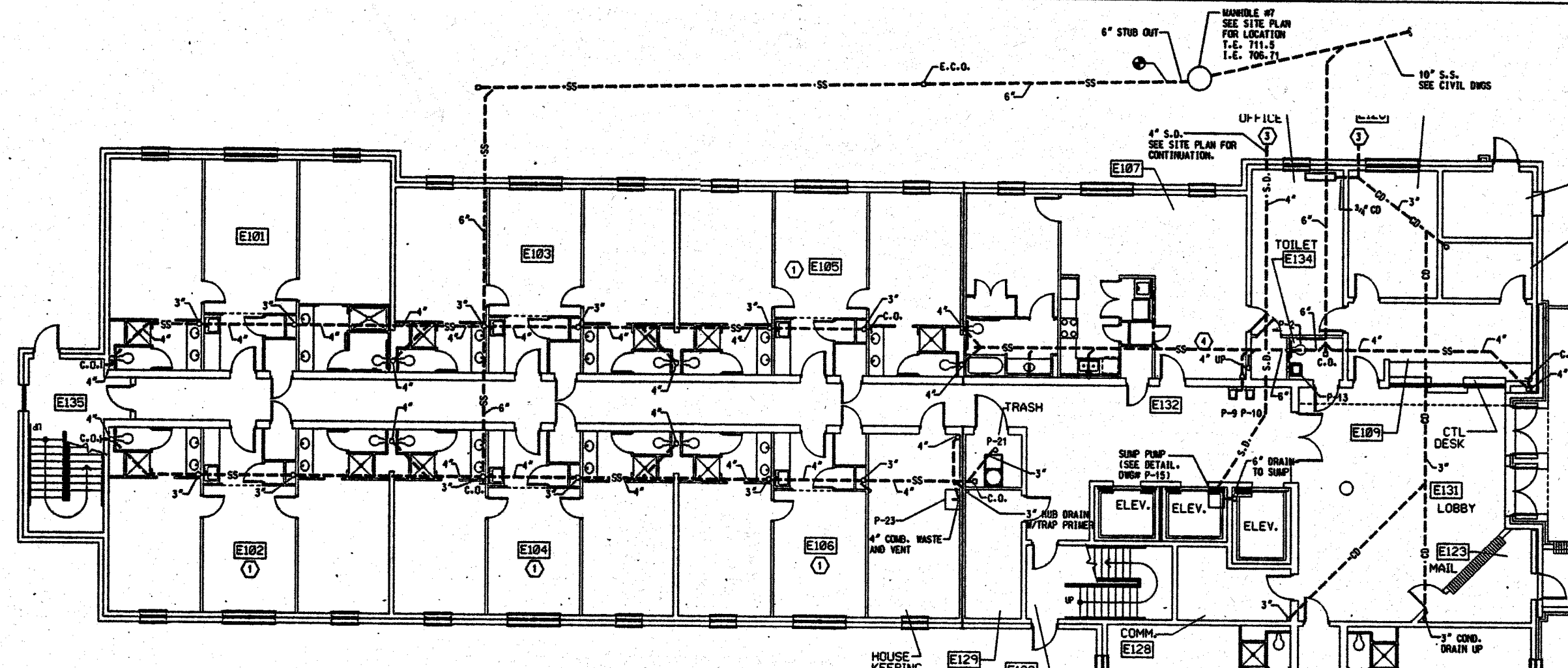
PLUMBING - UNDERGROUND FLOOR PLAN - PART 'A'
