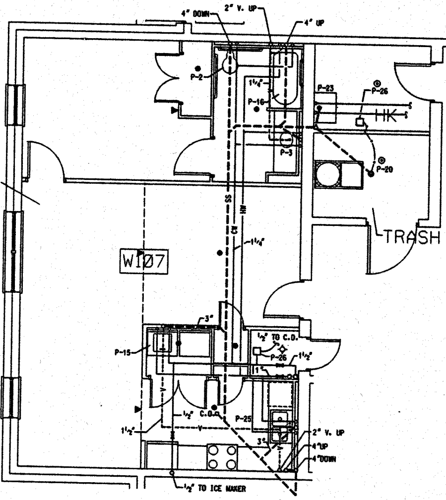
PLUMBING RESIDENT SUITE PLAN W107
