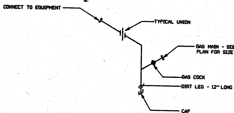
TYPICAL GAS CONNECTION DETAIL SCALE: NONE
