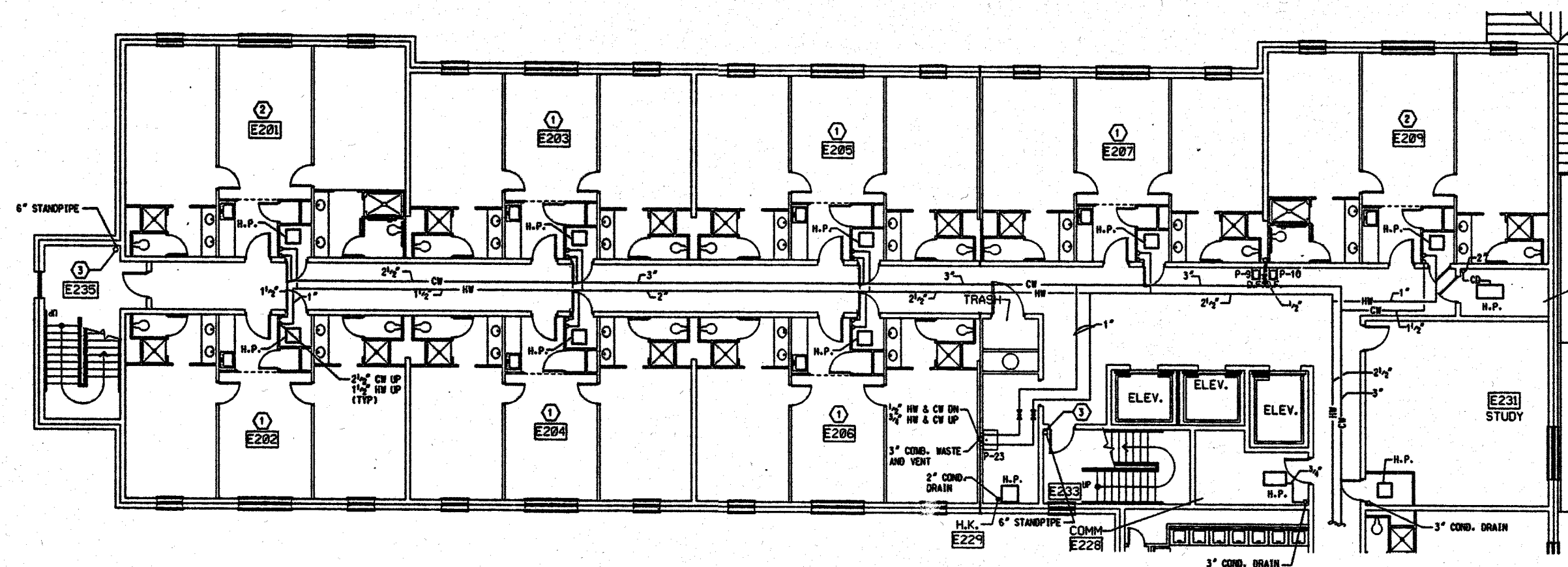
PLUMBING - SECOND FLOOR PLAN - PART 'A'
