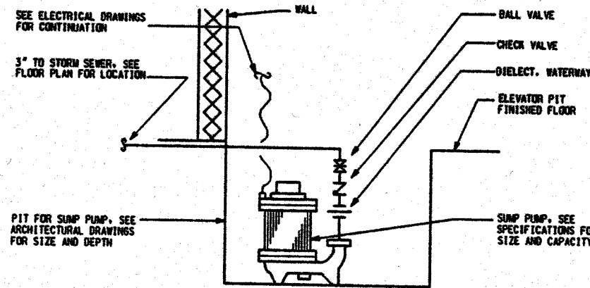
ELEVATOR SUMP PUMP DETAIL SCALE NONE
