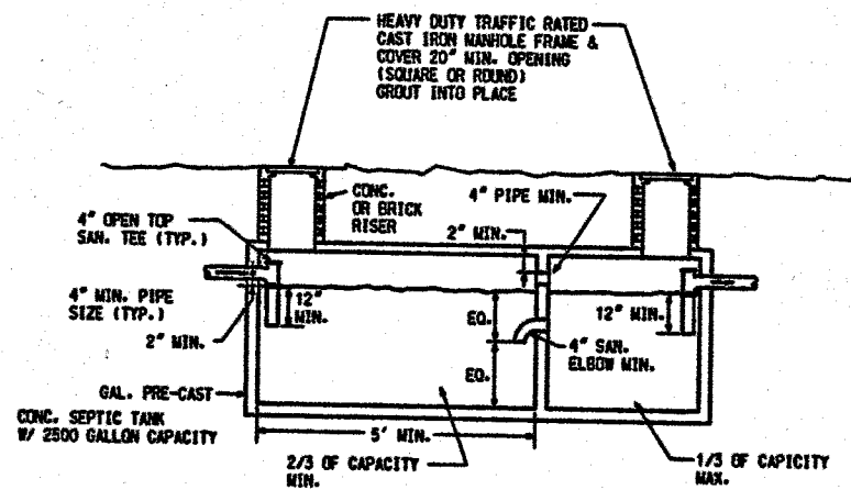
GREASE TRAP DETAIL SCALE: NONE
