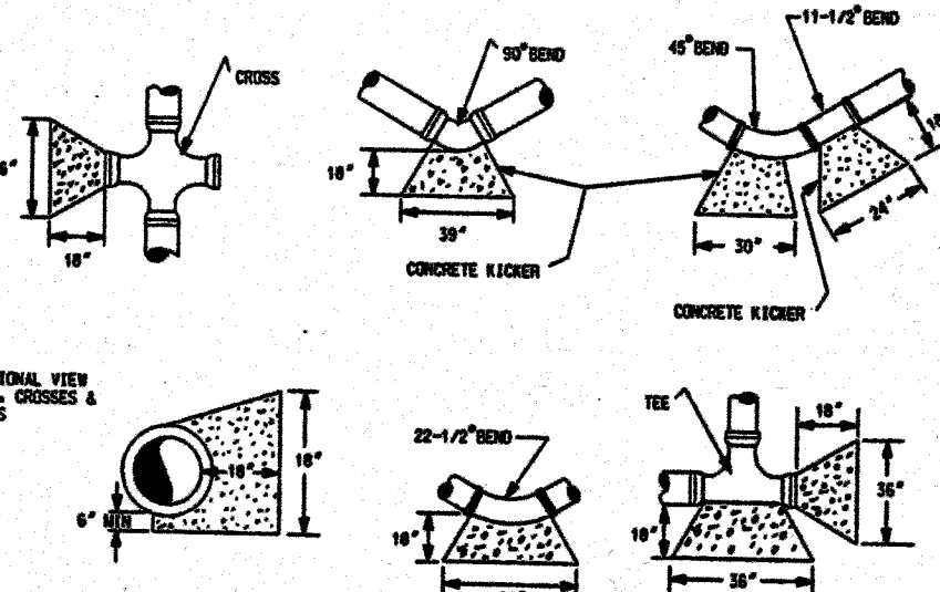
CONCRETE THRUST BLOCK DETAILS SCALE: NONE
