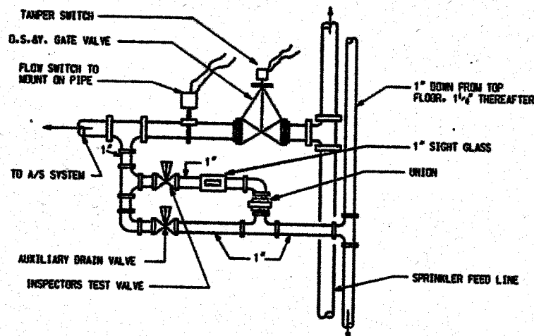
AUTOMATIC SPRINKLER CONTROL VALVE SCALE: NONE
