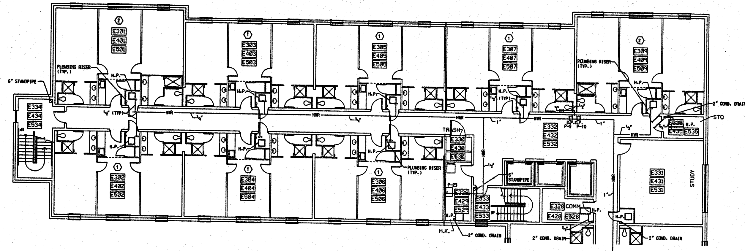
PLUMBING - THIRD, FOURTH, FIFTH FLOOR PLAN - PART 'A'
