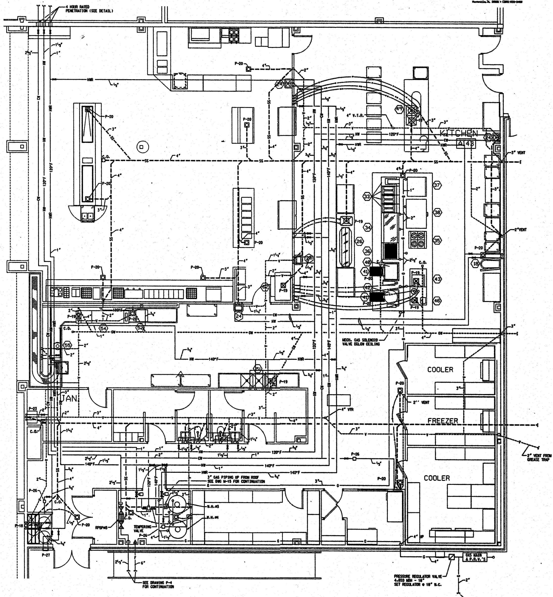
PLUMBING KITCHEN PLAN
