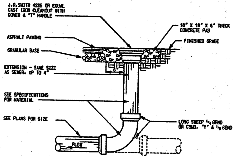
EXTERIOR CLEANOUT DETAIL SCALE: NONE
