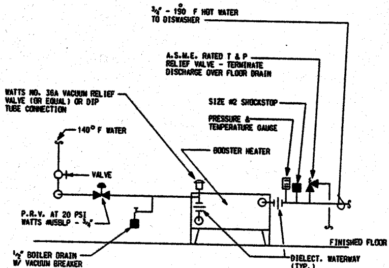
BOOSTER HEATER PIPING SCHEMATIC SCALE: NONE NOTE: VERIFY PIPING ARRANGEMENT WITH BOOSTER HEATER SUPPLIER
