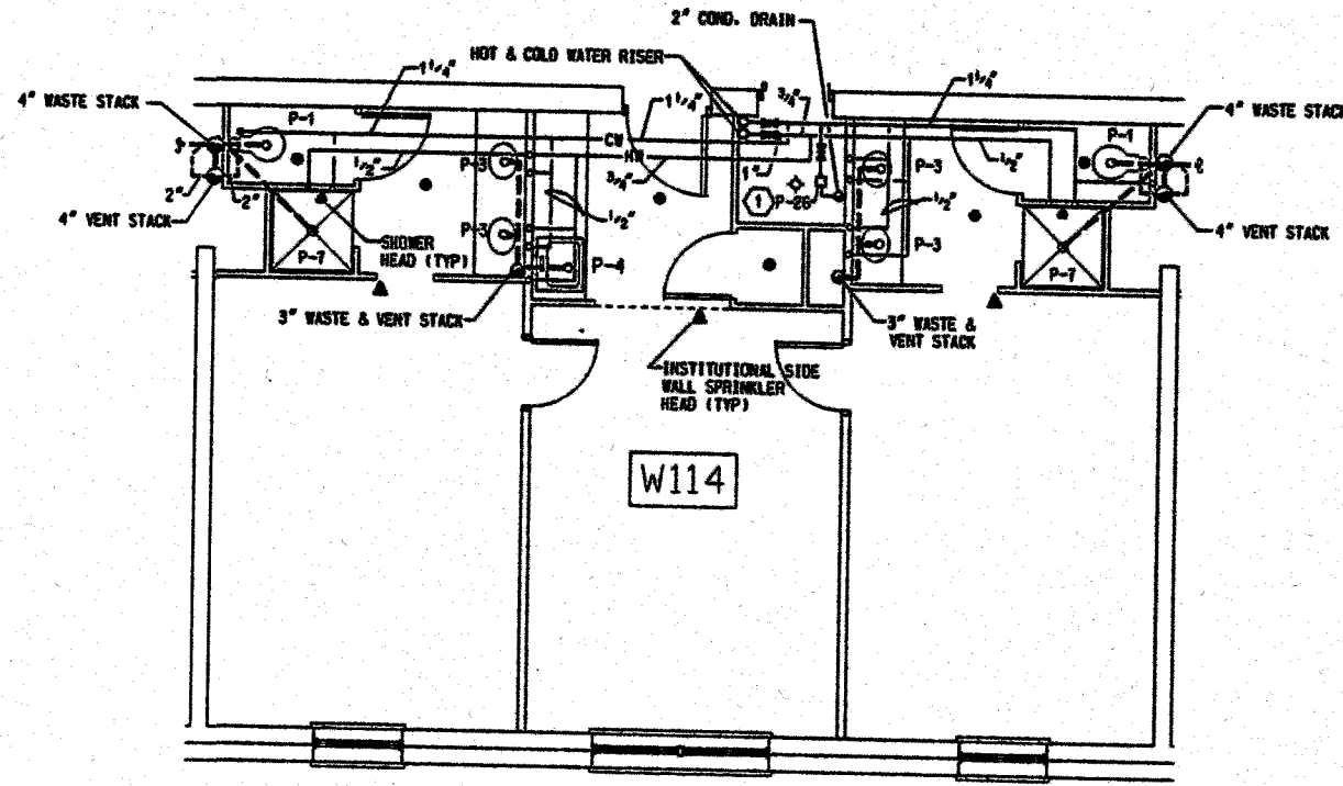
PLUMBING TYPICAL SUITE PLAN
