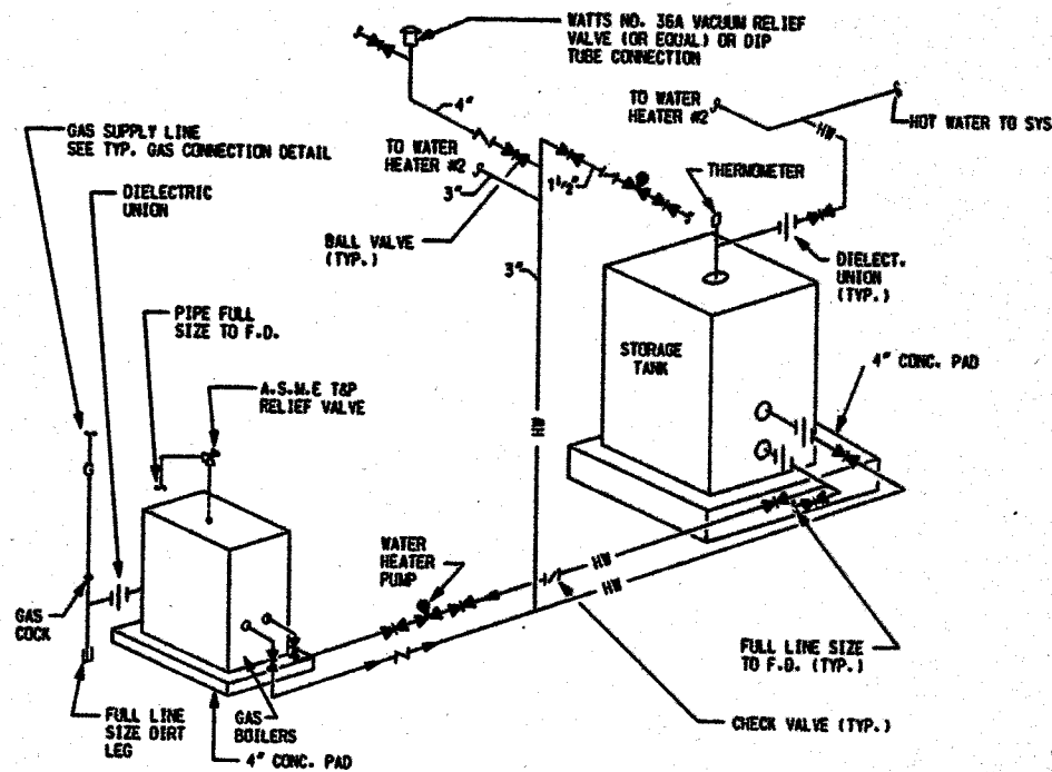
WATER HEATER #1 & #2 DETAIL SCALE NONE
