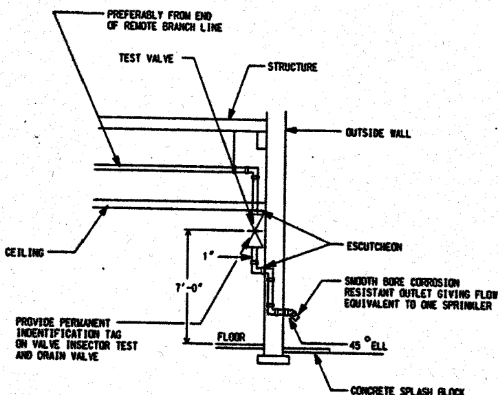
INSPECTOR'S SPRINKLER TEST PIPE SCALE: NONE
