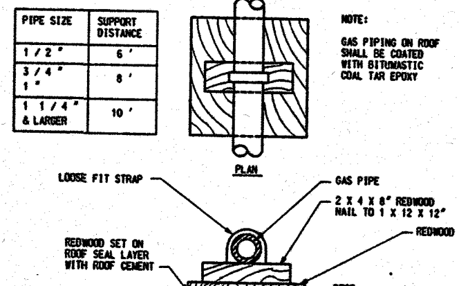
GAS PIPING ON ROOF DETAIL SCALE: NONE
