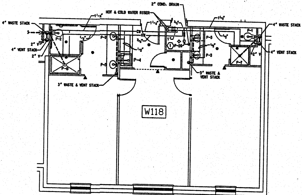
PLUMBING TYPICAL ACCESSIBLE SUITE
