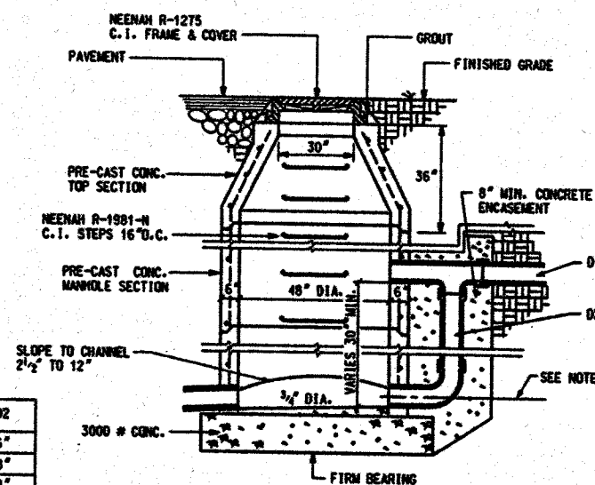
DROP MANHOLE DETAIL SCALE NONE
