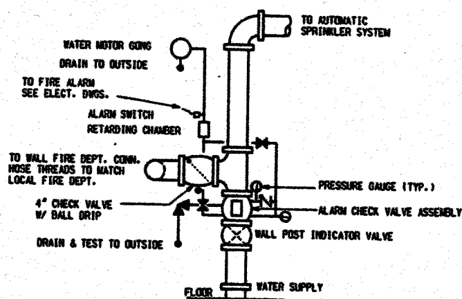
AUTOMATIC SPRINKLER ENTRANCE DETAIL (WET) SCALE: NONE
