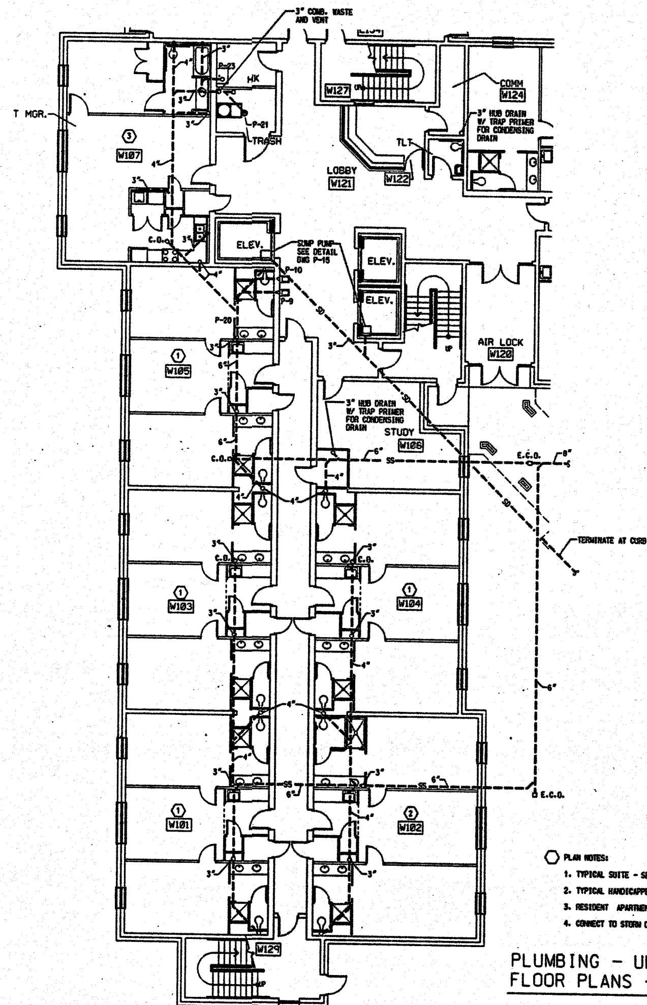
FLOOR PLAN - PART 'C'
