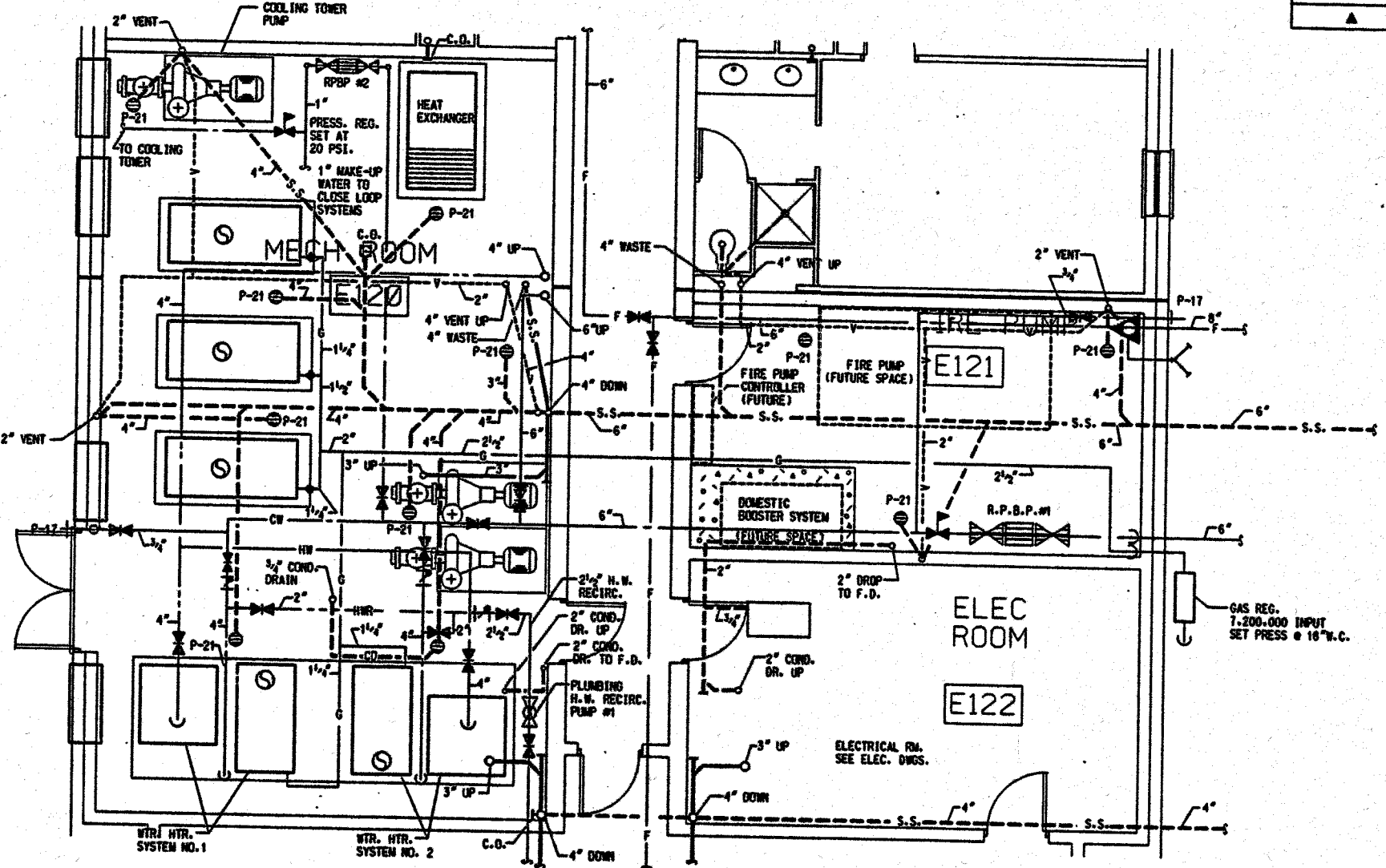
PARTIAL FLOOR PLAN
