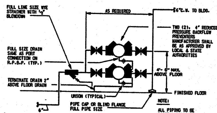
REDUCED PRESSURE BACKFLOW PREVENTER DETAIL SCALE NONE
